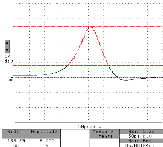
AVH-S-1-P Output, 100 kHz, 5V/div, 50 ps/div.
